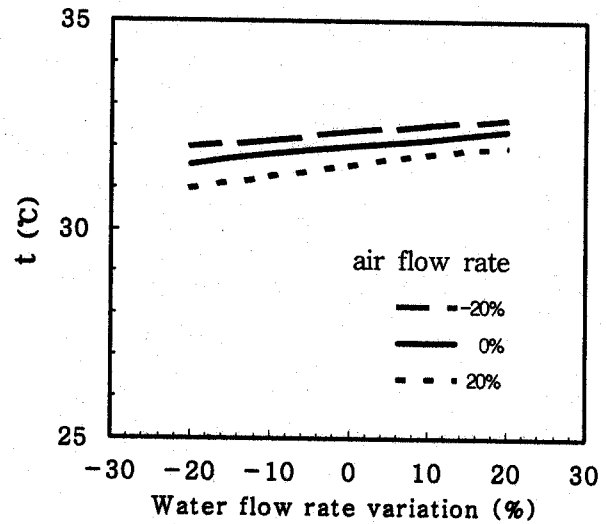
Fig. 4 Effect of water circulation rate on the exit water temperature.
