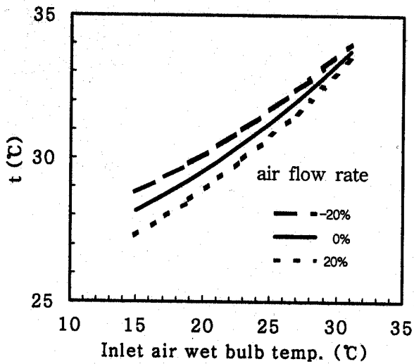
Fig. 2 Effect of wet bulb temperature on the exit water temperature.
