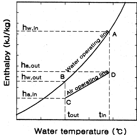
Fig. 1 Enthalpy-temperature diagram of air and water.
