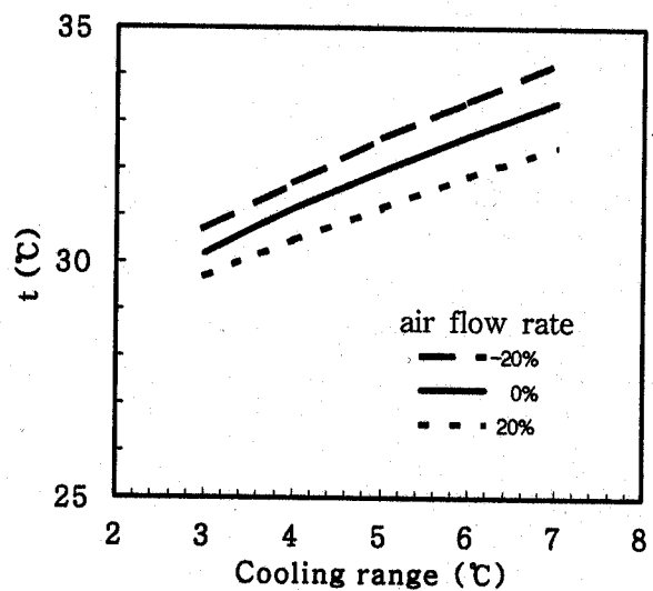
Fig. 3 Effect of cooling range on the exit water temperature.
